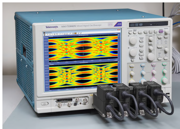
DP070E Series Optical probes using the TekConnect channel on a MSO73304DX Oscilloscope
