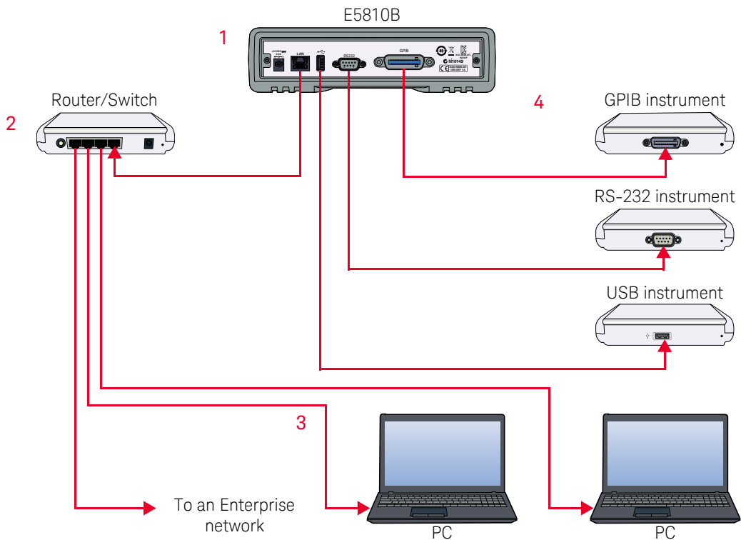
Figure 4-1 Troubleshooting overview
