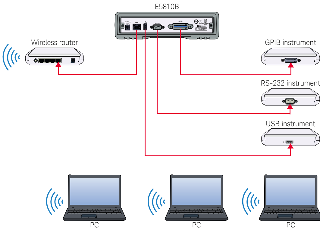
Figure 2-7 Connecting the E5810B to a wireless router
