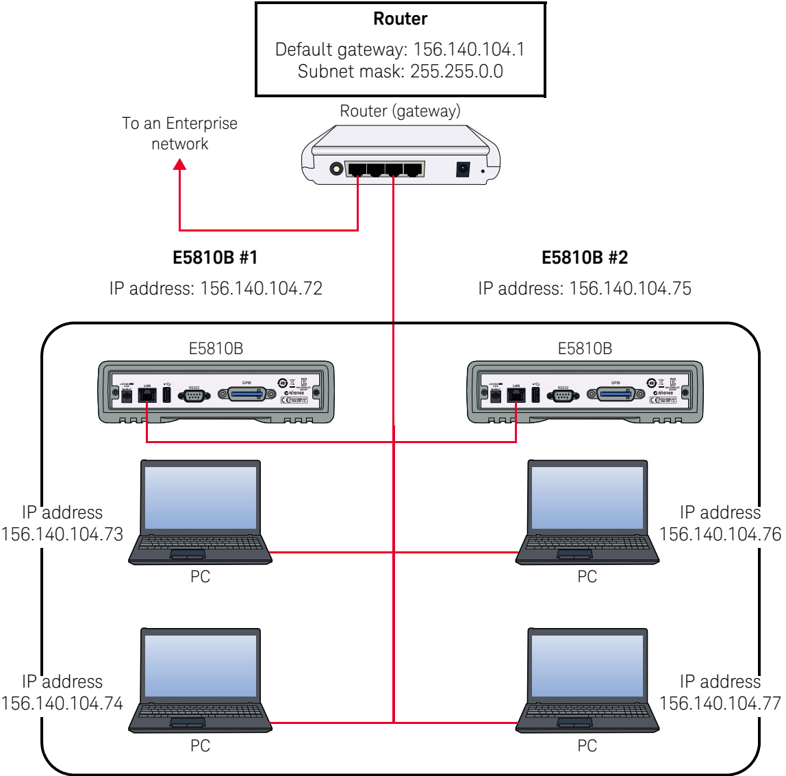
Figure 1-7 Typical network IP addressing
