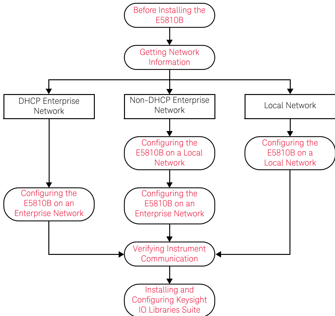
Figure 2-1 Installation flowchart
