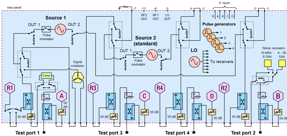
Figure 8. 4-Port N5247B Option 423 with 029
