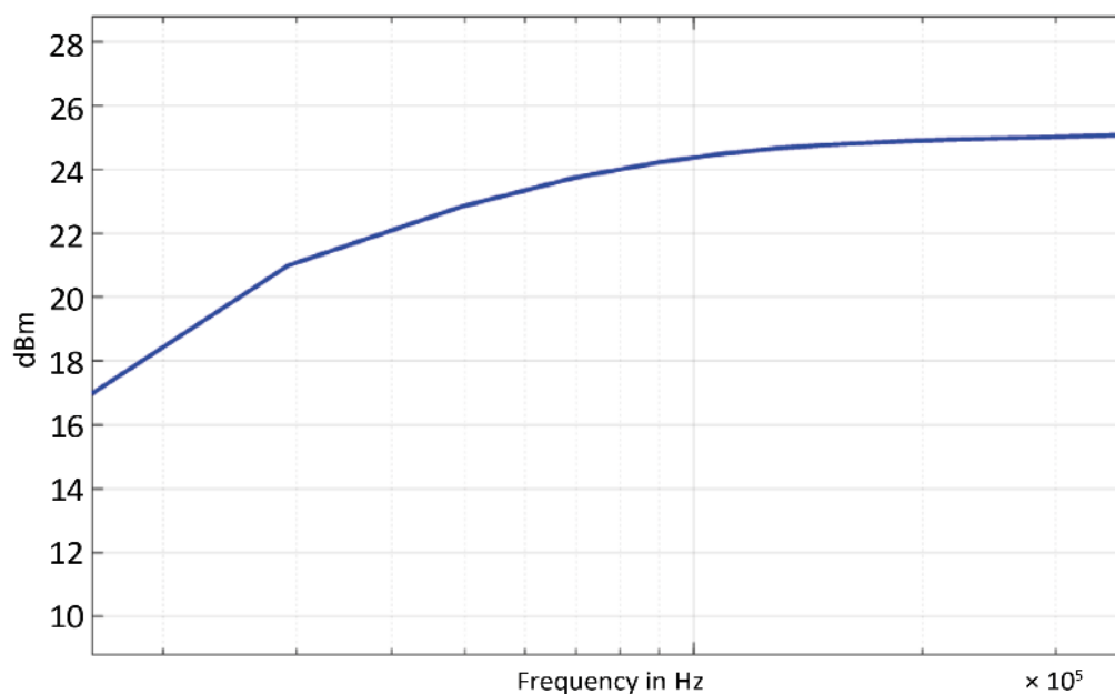
Figure 1. Nominal maximum output power, 9 kHz to 1 MHz, with Option 1EA
