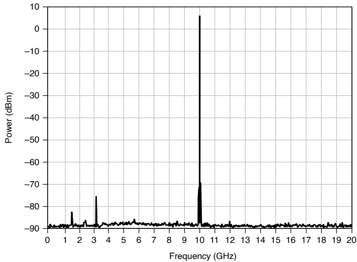
Figure 6. PXle-5654 with PXle-5696 Typical Spectrum at 10 GHz
