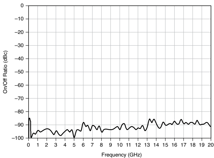
Figure 13. Pulse Modulation On/Off Ratio
