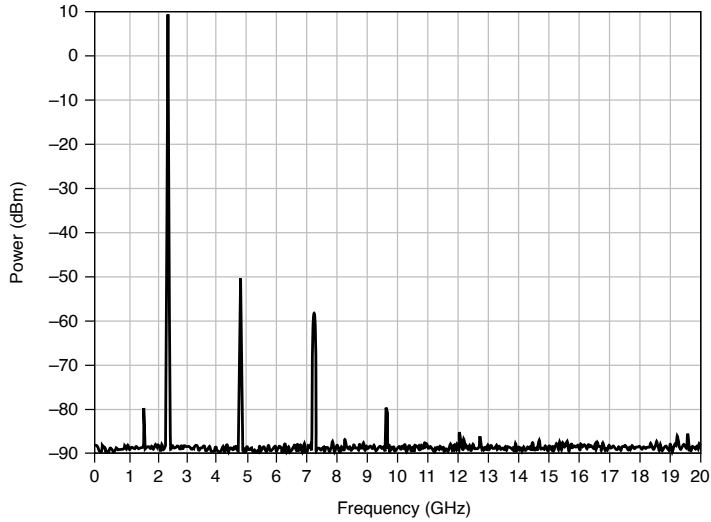
Figure 4. PXIe-5654 with PXIe-5696 Typical Spectrum at 2.4 GHz
