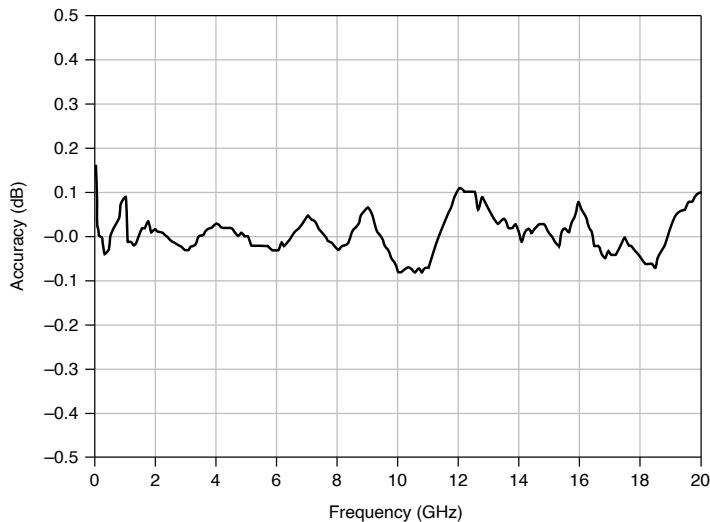
Figure 8. PXle-5654 with PXle-5696 Typical Power Accuracy at -40 dBm
