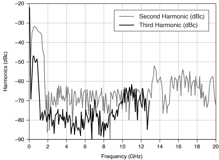
Figure 2. PXIe-5654 with PXIe-5696 Typical Harmonic Levels at +8 dBm Output Power
