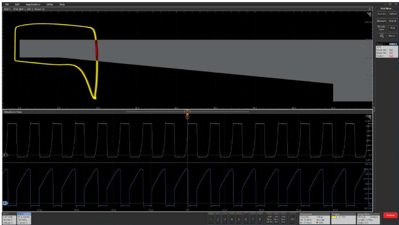
Safe Operating Area (SOA) plot with mask helps verify the switching devices are staying within their SOA envelope under changing operating conditions.
