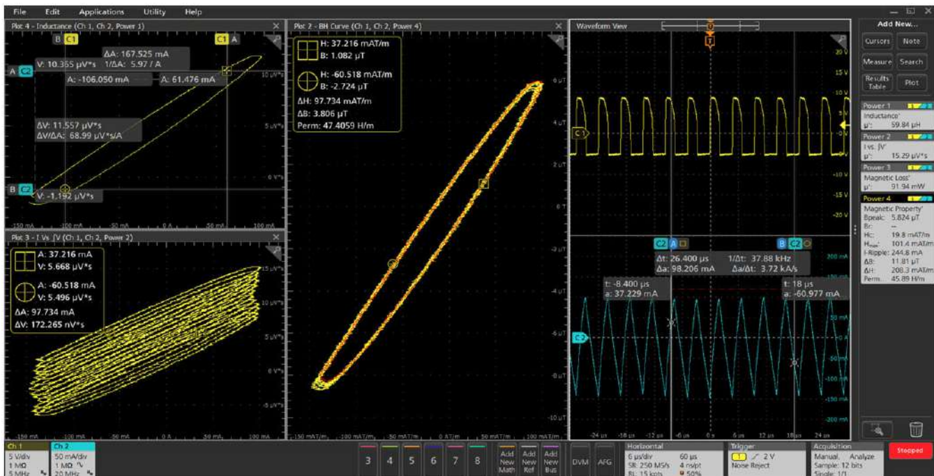
Magnetic Analysis measurement with B-H curve, I vs. \int V , and Inductance plots
