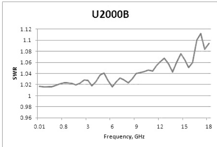
Typical SWR for U2000B sensor (25 °C ± 10 °C)
