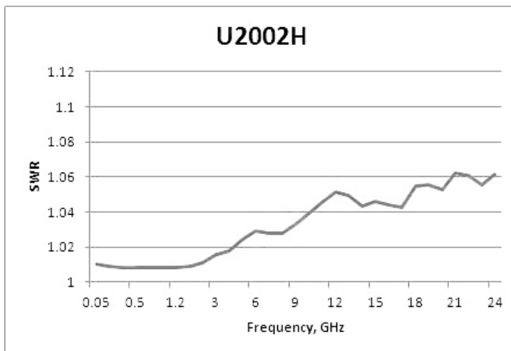
Typical SWR for U2002H sensor (25 °C ± 10 °C)
