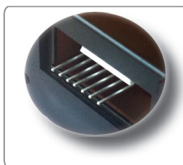
0-FLUCS CT-100/CT-150 7-pin strip connector for PCB
