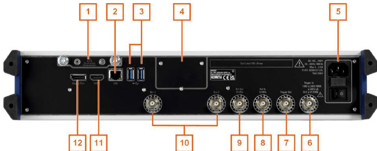
Figure 5-2: Rear panel view of MXO 5C series oscilloscope
