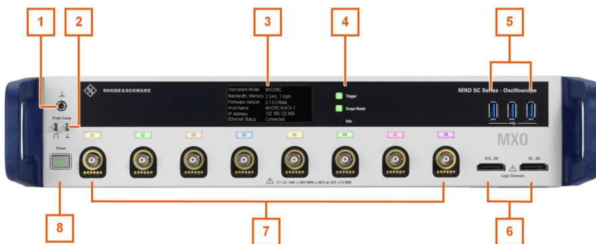
Figure 5-1: Front view of MXO 58C with 8 input channels
