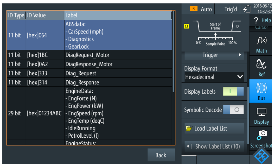
Figure 9-27: Display of a CAN DBC file
