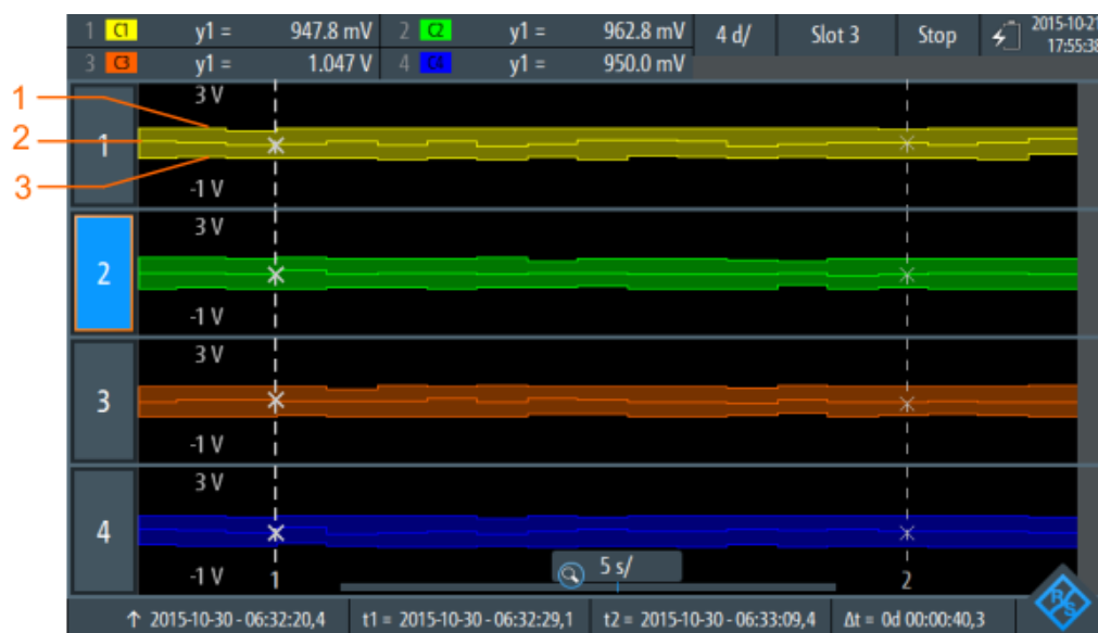
Figure 8-6: Logger zoom with summarized data
