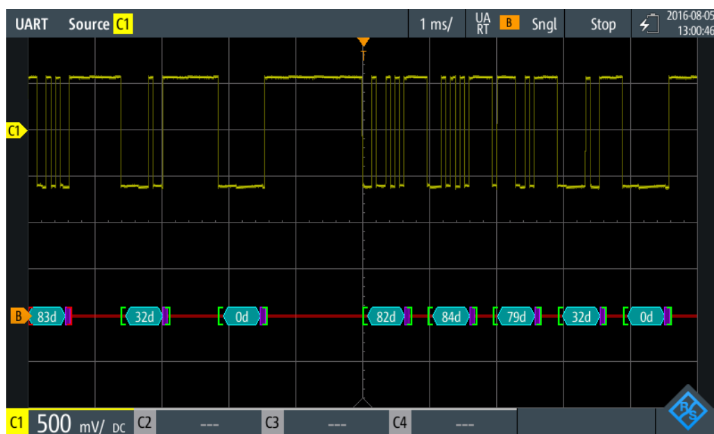
Figure 9-20: Comb display of a decoded UART signal, triggered on the start bit
