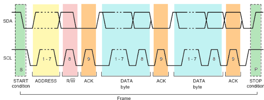
Figure 9-7: I2C write access with a 7-bit address
