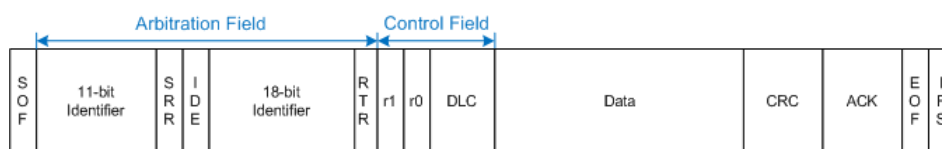
Figure 9-24: CAN extended frame
