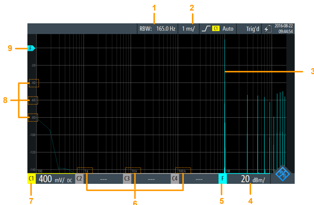
Figure 6-1: FFT display
