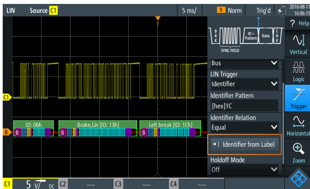
Figure 9-36: Trigger on identifier "Left brake"
