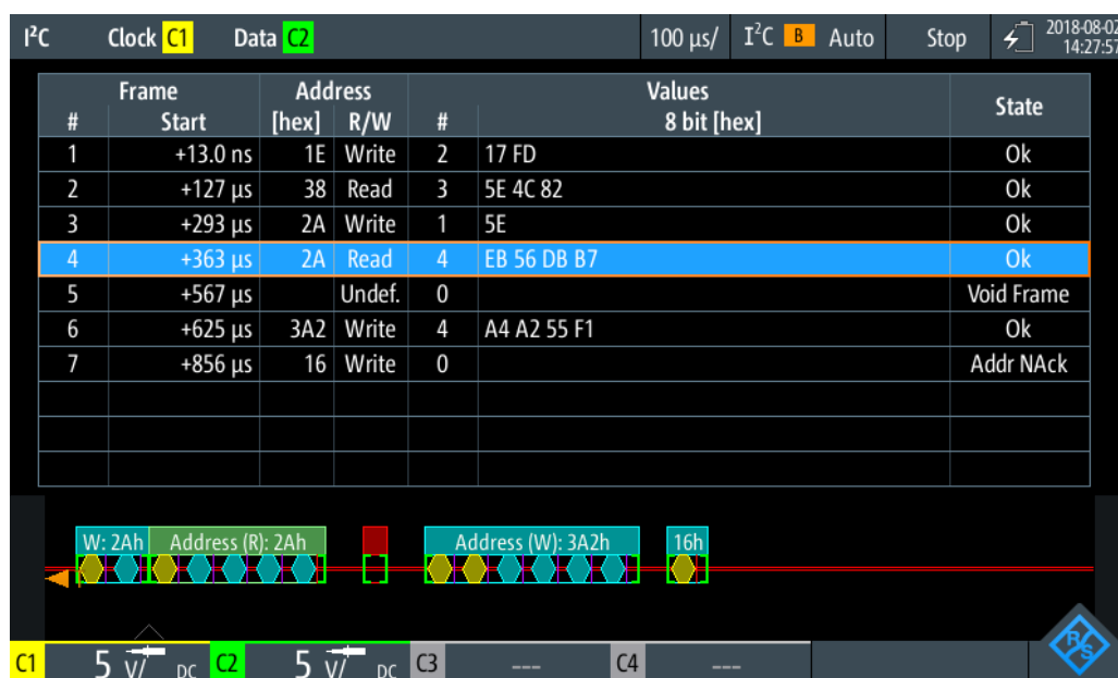
Figure 9-14: Decoded I²C signal in Protocol mode
