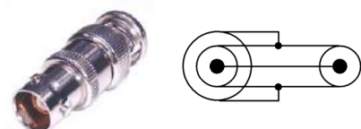
N1254A-102 Triax (f) to BNC (m) adaptor
