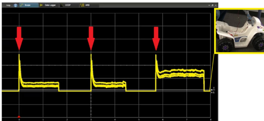
Figure 3. Example of a typical peak power surge waveform. The start-up current spikes as indicated by the red arrows each time the acceleration pedal on a toy electric vehicle (figure subset) is applied.
