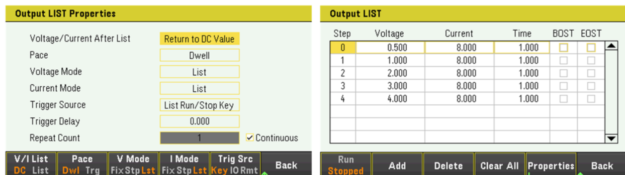
Figure 9. LIST mode output programming user interfaces.
