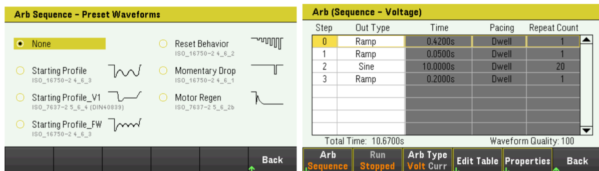
Figure 12. Automotive ISO preset library readily to be loaded (left). Each of the ISO preset waveforms are segmented into steps that allow users to easily go into the specific segments and modify the parameters according to user test cases. Additional steps can be added or removed for greater flexibility (right).
