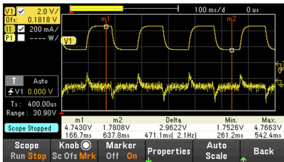
Figure 10. Scope view.
