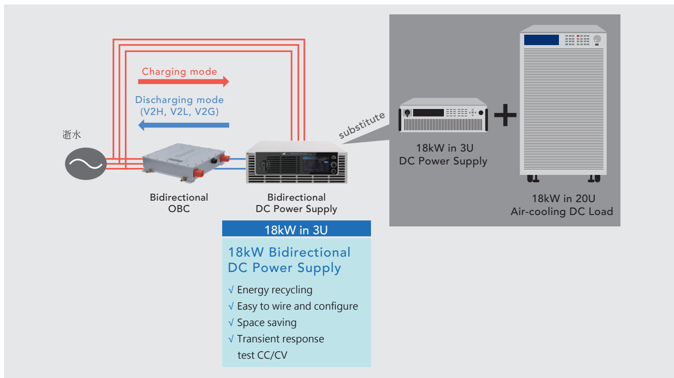
Bidirectional on-board charger testing configuration
