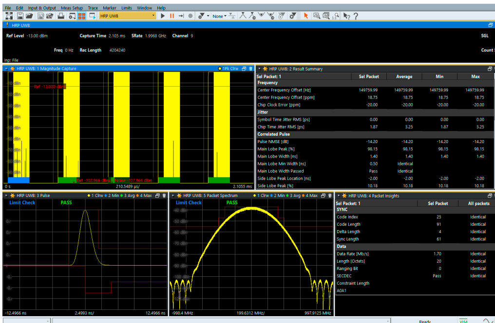
Analysis of a 499.2 MHz wide HRP UWB signal.
