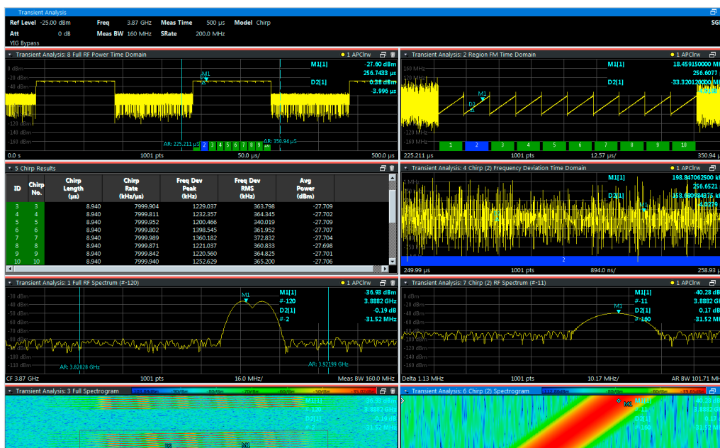
Analysis of a chirp signal with different measurement windows.
