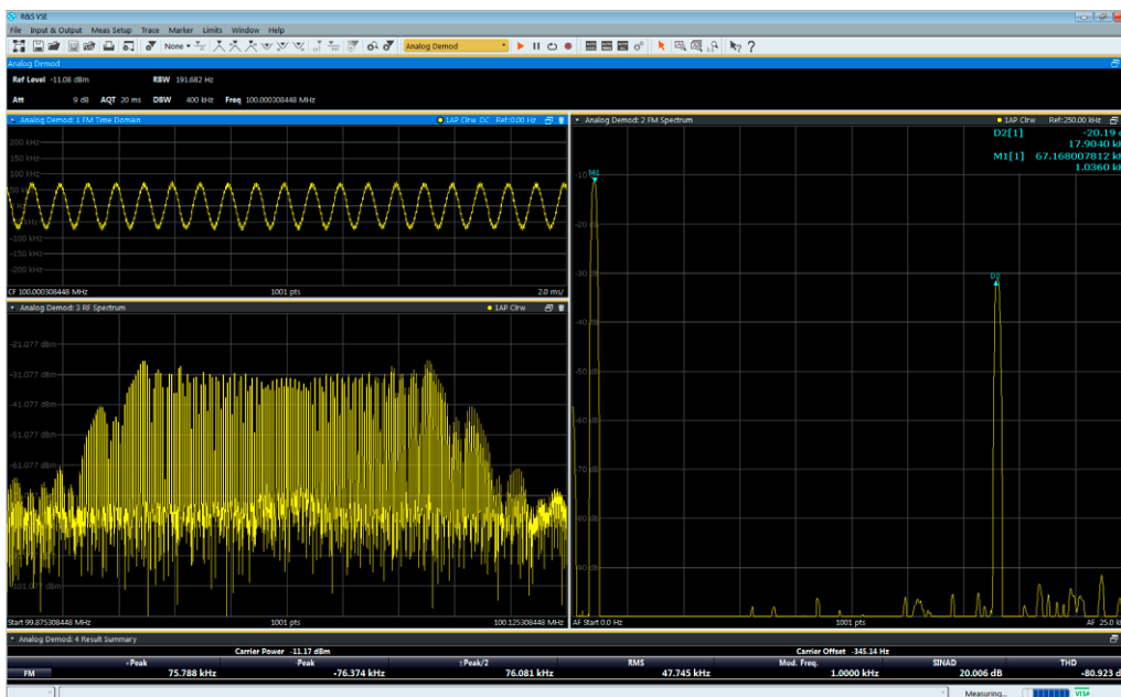
FM signal displayed in time domain, RF spectrum and FM spectrum.
