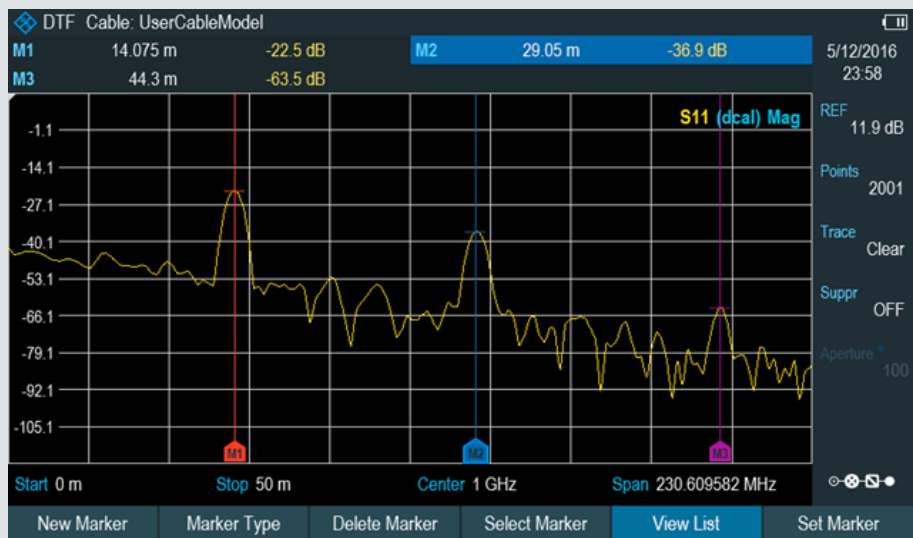
Distance-to-fault measurement
