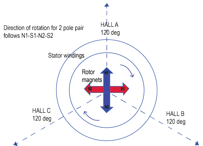
Direction information interpreted from the Hall sensor outputs.
