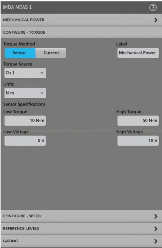
Configuration options for Mechanical Power measurement.
