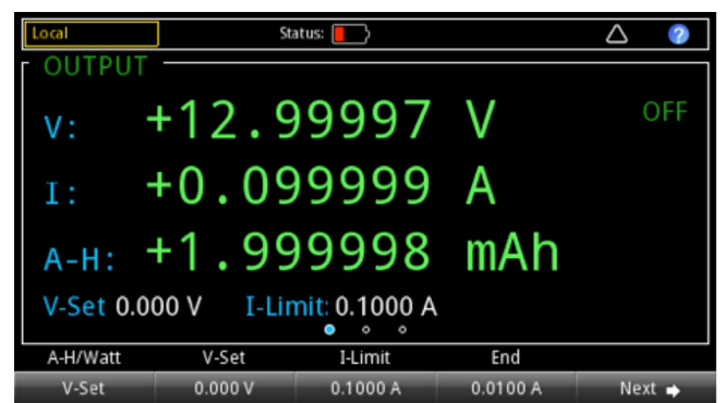
Figure 4. Battery test display.
