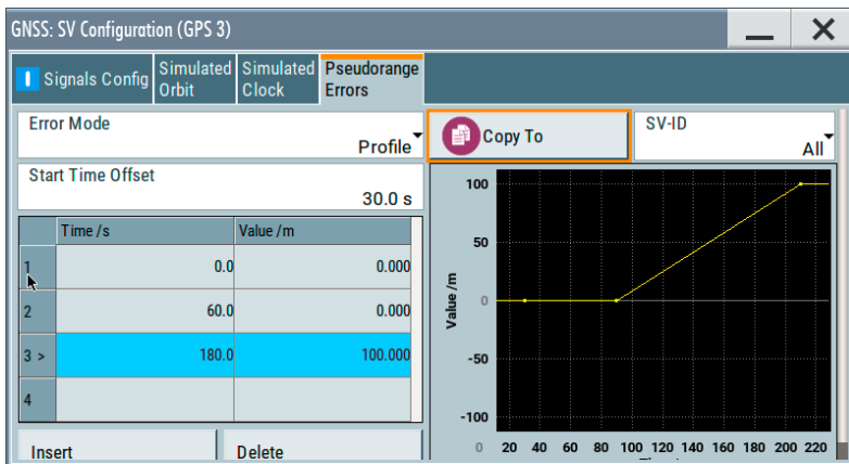
Simulation of a pseudorange ramp for SV 3 with the R&S®SMBV100B for testing the RAIM capabilities of a GNSS receiver
