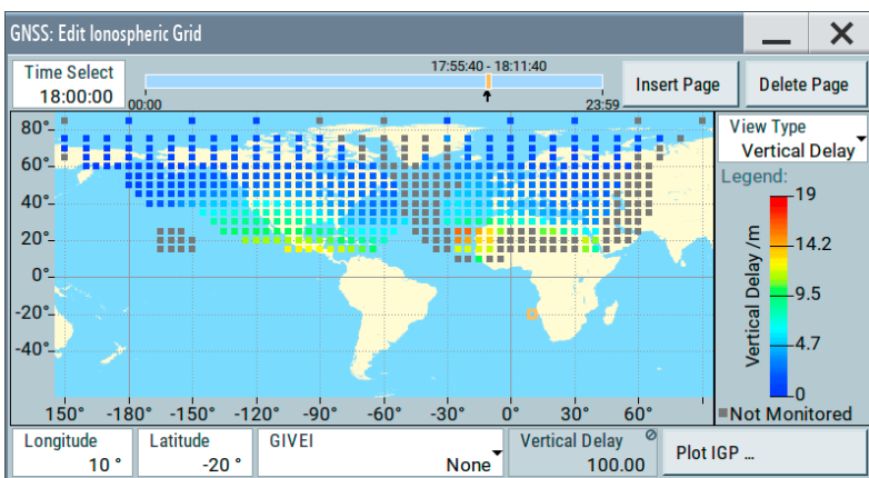
Configuration and simulation of ionospheric path delays with the R&S®SMBV100B
