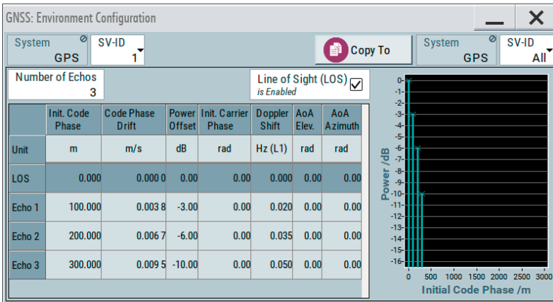
Simulation of multipath propagation for SV 1 with the R&S®SMBV100B. In addition to the line of sight, three reflections with different relative delays, relative amplitudes and relative Doppler shifts are present
