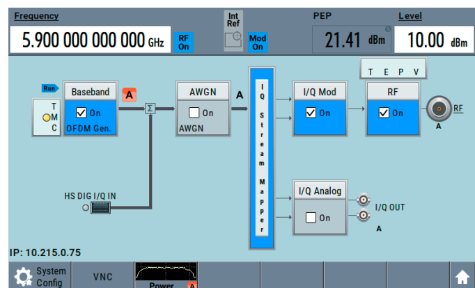
Functional block diagram of the R&S®SMBV100B
