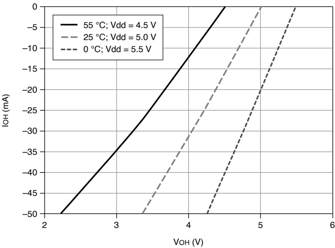
Figure 3. P0.<0..7>: I_{OH} versus V_{OH}
