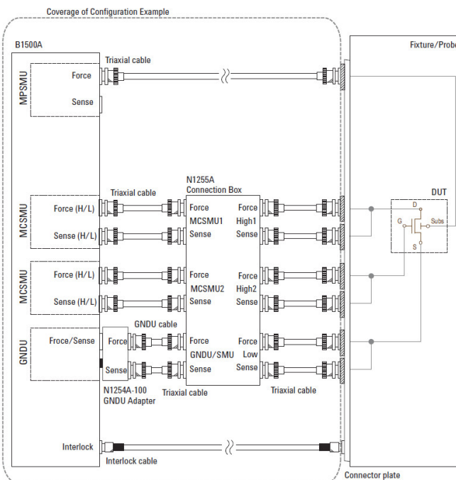
Example-6. For 50 \mu s pulse using two MCSMU for 4-terminal device
