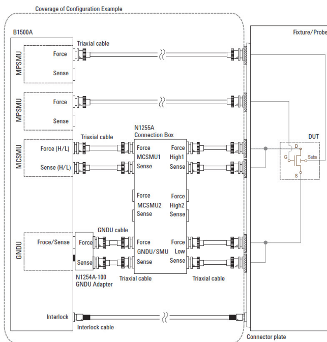
Example-5. For 50 \mu s pulse using one MCSMU for a 4-terminal device
