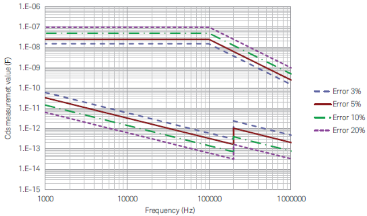
Cds measurement accuracy 3-terminal Cgs:Cds:Cgd = 1:1:1
