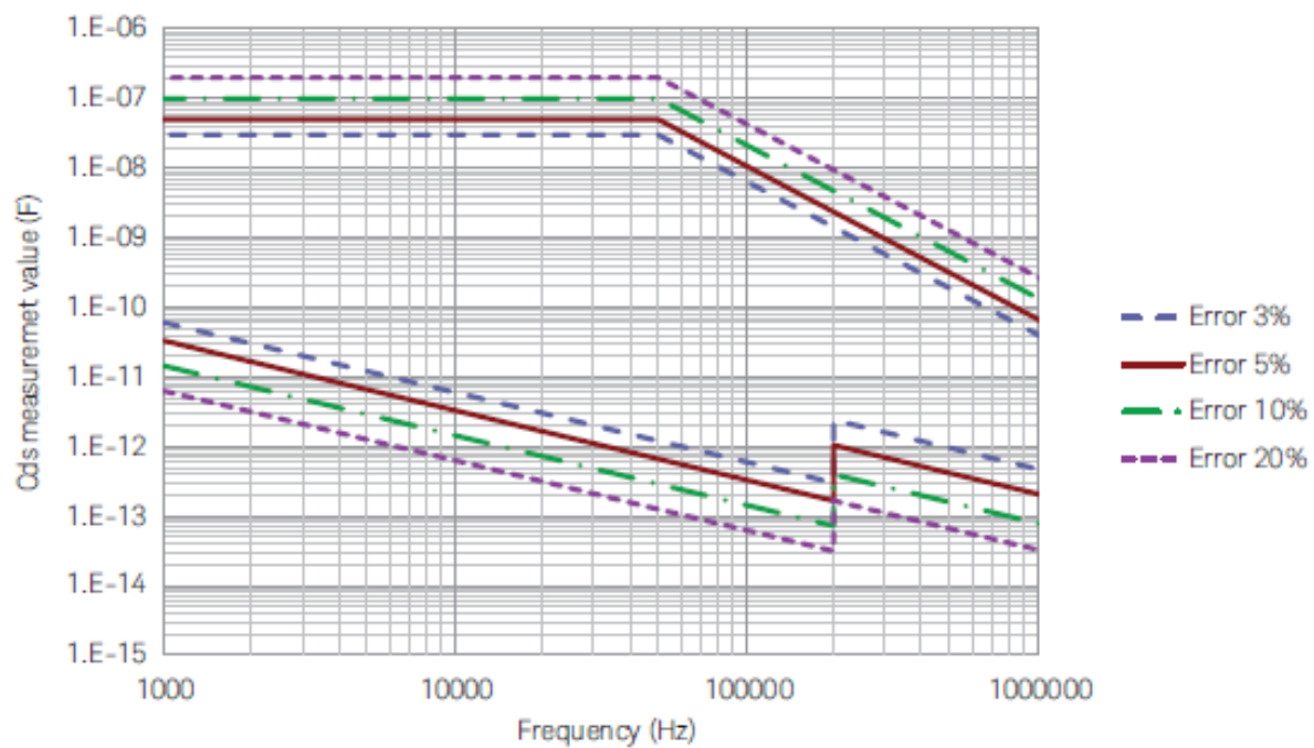
Cds measurement accuracy 3-terminal Cgs:Cds:Cgd = 1:0.1:0.01
