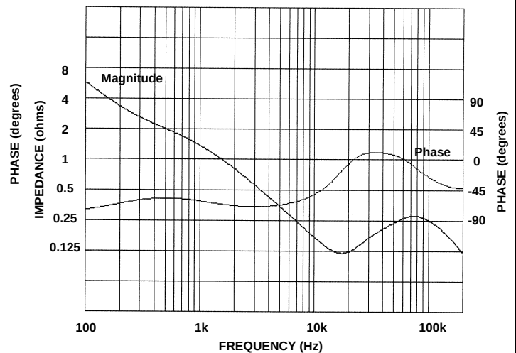
Model N6762A, CC Mode, @50V, 2A
