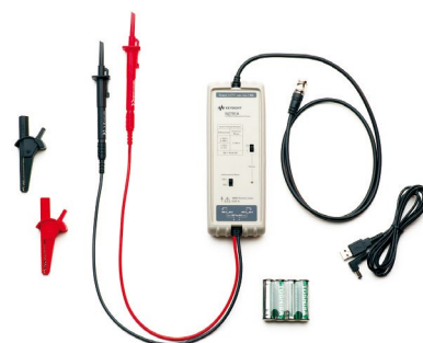
N2791A 25-MHz, 700-V differential probe
