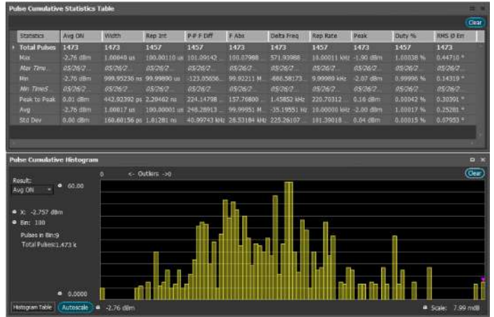
Cumulative statistics provides timestamps for Min, Max values as well as Peak to Peak, Average and Standard deviation over multiple acquisitions, further extending the analysis. Histogram shows you outliers on the right and left.
