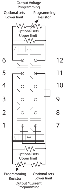
Fig.6-2: J1-Remote Resistor Programming Connection
