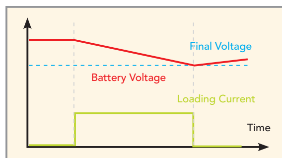
Battery Discharge Testing
