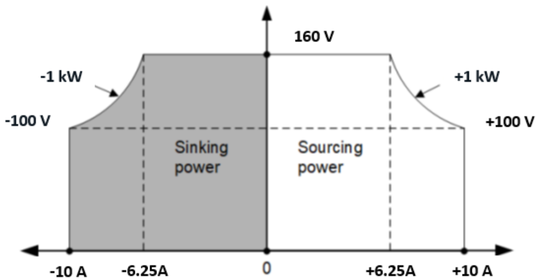
Figure 13. Output quadrants of the MP4361A
