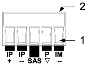
Analog connectors in E436xA modules
