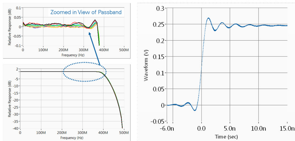
Figure 7. This graph shows the frequency and step response of a typical PXle-5164 oscilloscope on the 50 Ohm path up to the full bandwidth. The response of all ranges and channels of one module are superimposed and the maximum deviation in the passband is 0.022.
