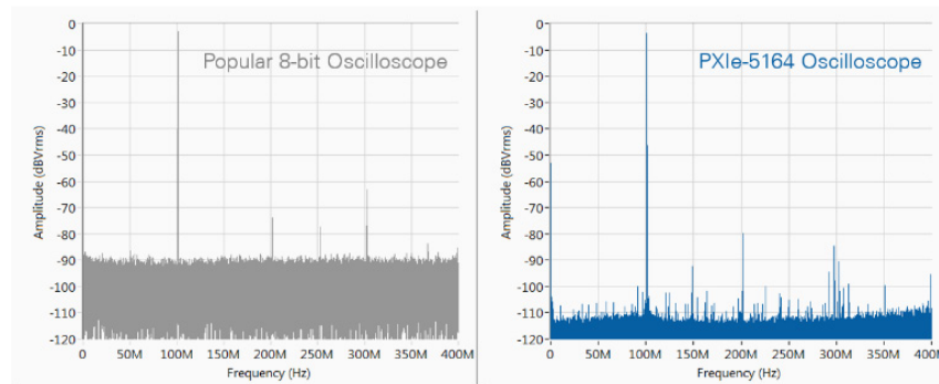
Figure 6. By comparing the spectral results of a popular 8-bit box oscilloscope with the PXle-5164 oscilloscope, you can see the noise floor of the PXle-5164 oscilloscope is a significant 22 dB lower.
