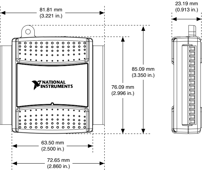
Figure 2. USB-6009 Dimensions
