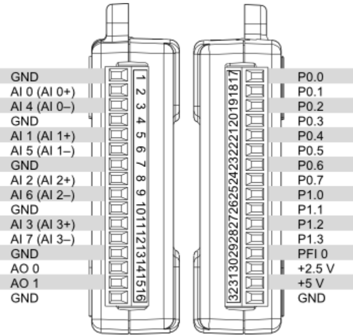
Figure 1. USB-6009 Pinout
