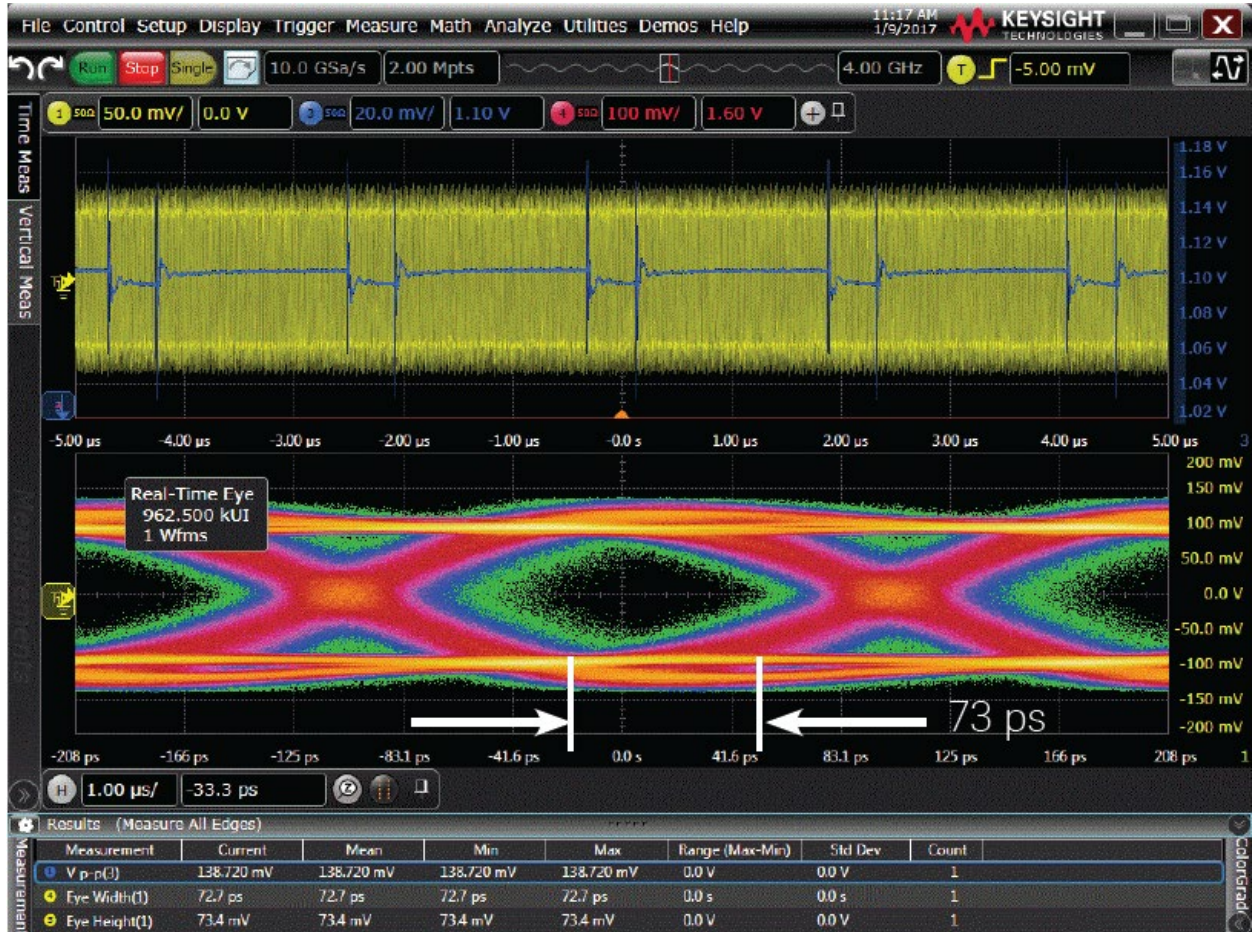
Figure 18. Eye diagram of FPGA serial data effected by DC supply noise.
