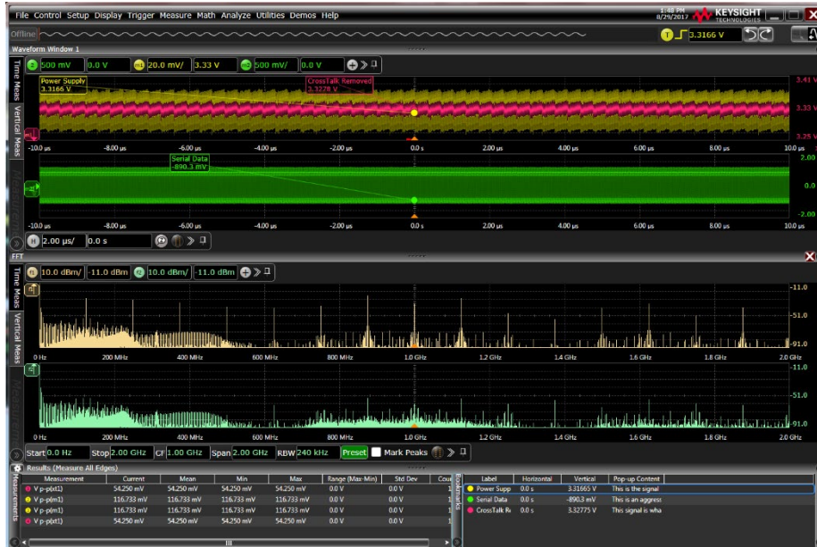
Figure 24. Output from the D9110POWA PI application showing a reduction in the noise on the 3.3 V supply after the effects of the switching loads were removed.
