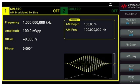
Figure 6. AM modulated with a standard sine wave
