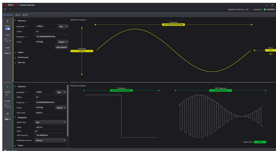
Figure 7. The PathWave BenchVue function generator app helps control function generators intuitively, load/design arbitrary waveforms, and build automated tests quickly.
