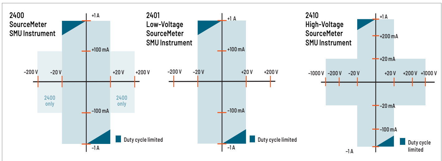
Series 2400 SourceMeter SMU Instruments
