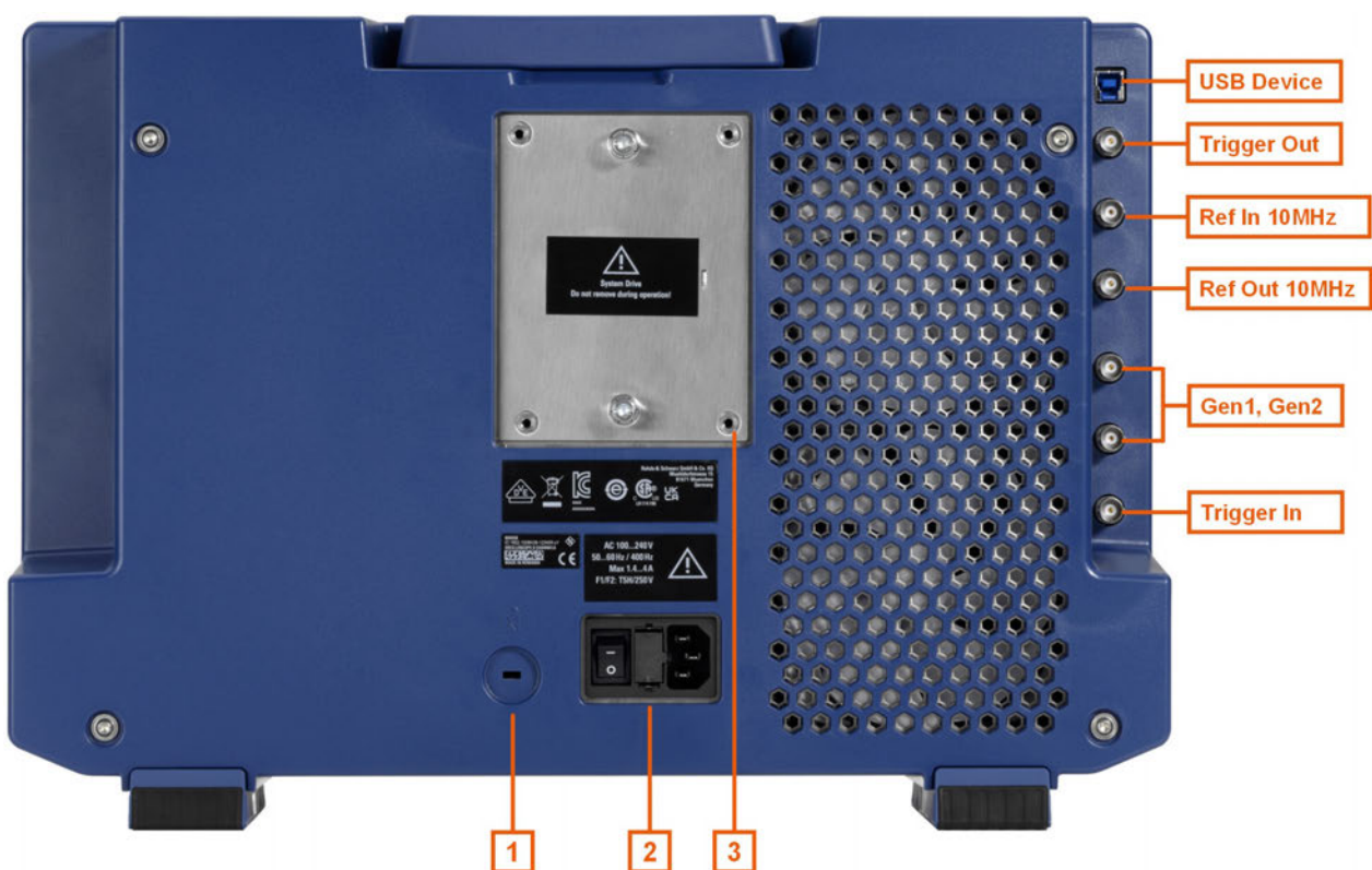
Figure 4-3: Rear panel view of R&S MXO 5
