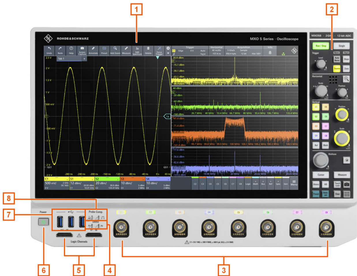
Figure 4-1: Front view of R&S MXO58, with 8 input channels
