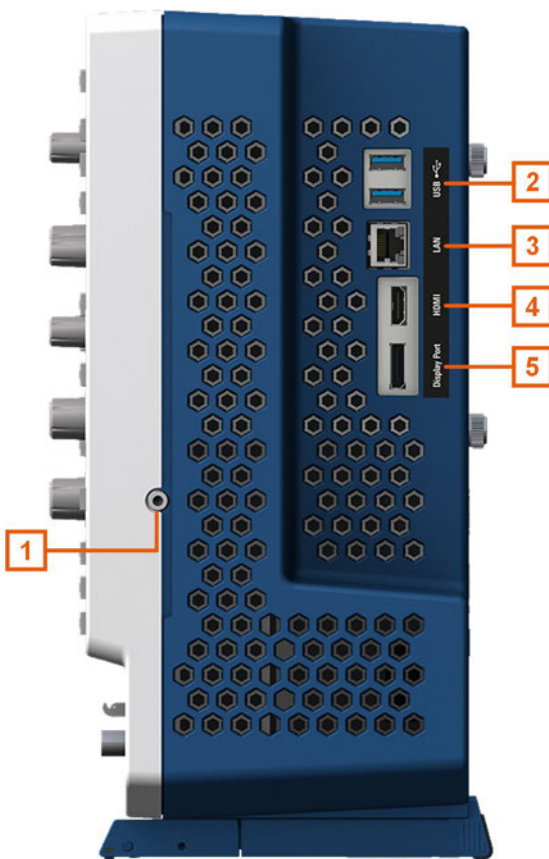
Figure 4-2: Side view of R&S MXO 5
