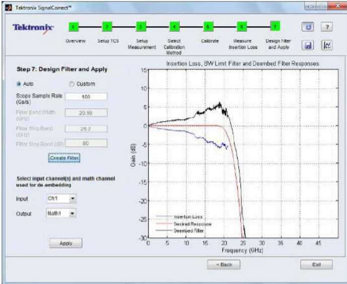
SignalCorrect creates a filter that you can apply to your oscilloscope inputs to de-embed your device or interconnect under test.
