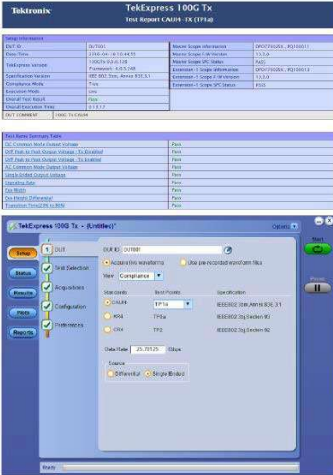
IEEE 802.3bj (KR4/CR4) and IEEE 802.3bm (CAUI4) Electrical Real Time Transmitter Compliance and Characterization Solution (option 100G-TXE) - TekExpress 100G-TXE automation provides turnkey testing and debug of 100G Ethernet's three most common electrical interfaces. Tools for 100G- KR4/CR4/CAUI4 are brought together in a single 100G-TXE option to support silicon designers and system designers as they perform KR4 and CR4 validation.
