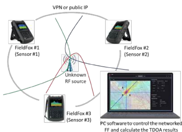
TDOA solution using three networked FieldFox analyzers and Windows PC software KSMS
