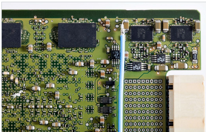
Pigtail cables do not limit the bandwidth of the probe and provide excellent connectivity right where the measurement has to be taken.
