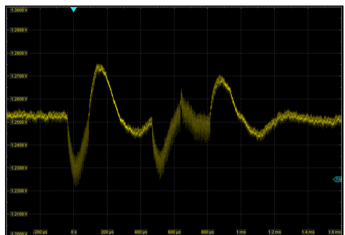
Load response measurement of a DDR4 power supply during initialization phase of the DDR memory.
