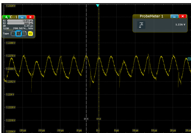
Measuring remaining ripple on a 1.2 V DDR4 power supply and accurately verifying the DC level with the R&S®ProbeMeter, a DC voltmeter integrated into the probe head.
