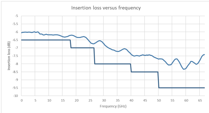
Figure 16. 11667D Insertion loss versus frequency (typical)
