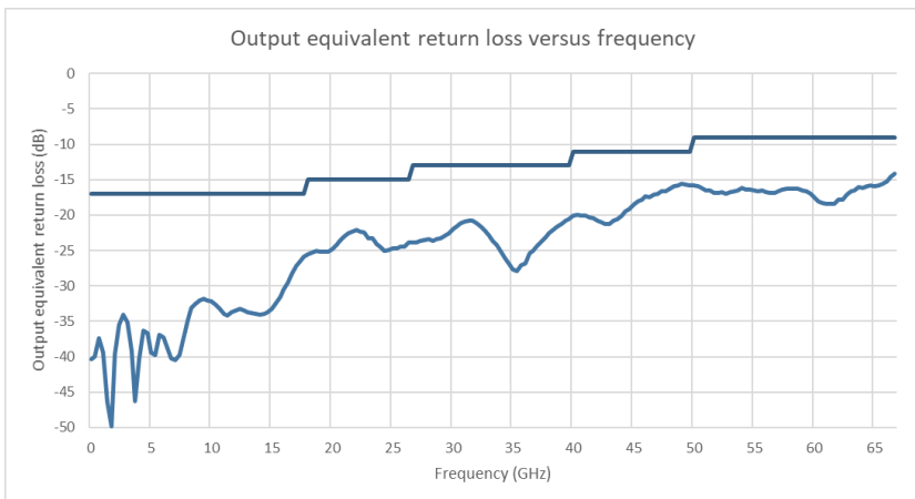
Figure 15. 11667D Output equivalent return loss versus frequency (typical)
