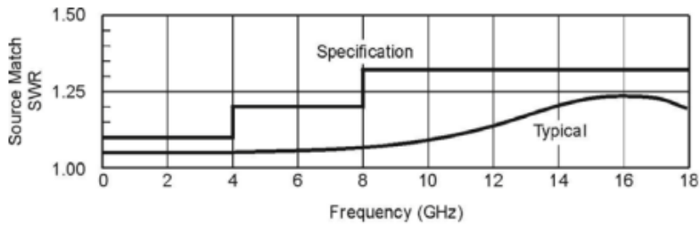
Figure 11. 11667A Leveling or ratio measurement source match (typical)
