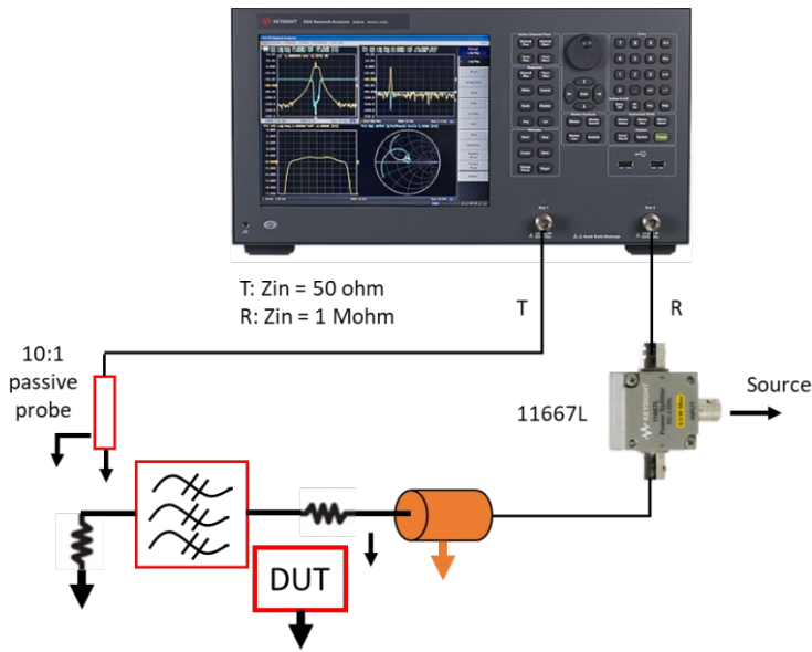
Figure 3. Non- 50-ohm LF filter measurement
