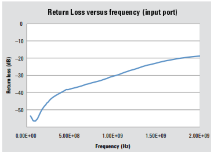
Figure 6. 11667L input port return loss versus frequency (typical)
