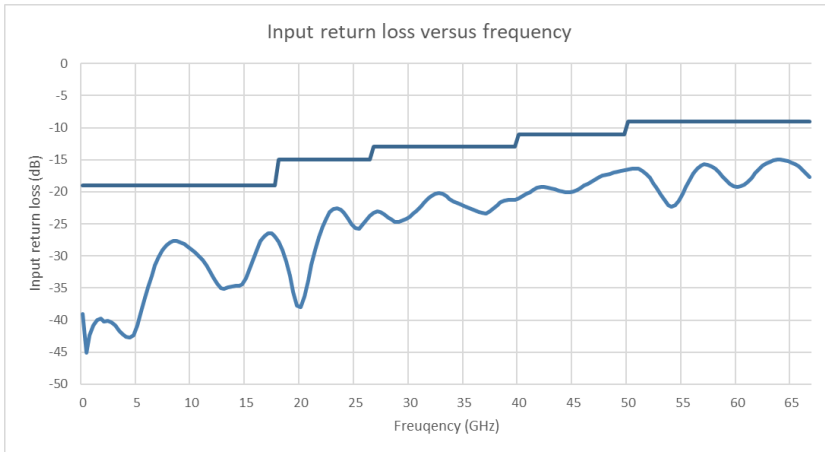
Figure 14. 11667D Input return loss versus frequency (typical)
