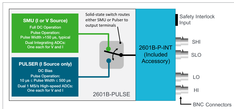
External Interlock/Connector box included with 2601B-PULSE
