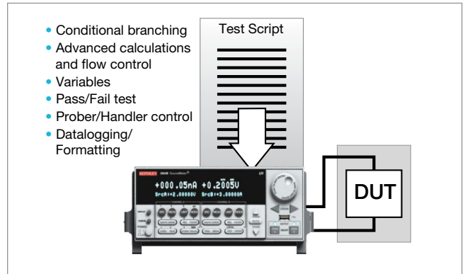
TSP technology executes complete test programs from the non-volatile memory of the 2601B-PULSE.
