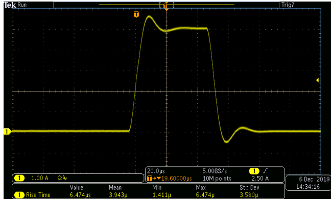
Typical pulse output from a competitive SMU with overshoot and 6.47 μs rise time.
