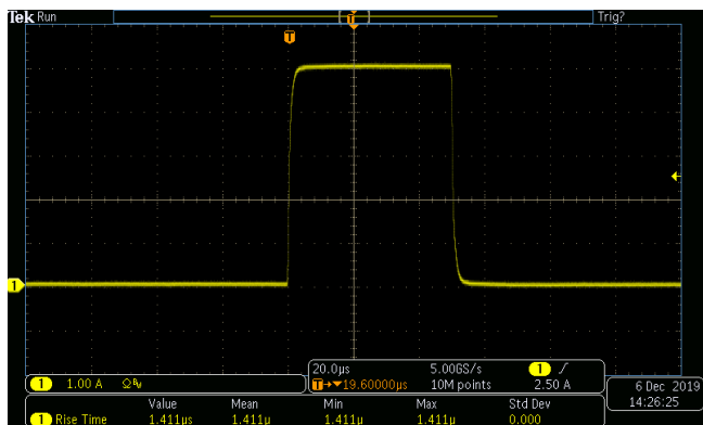
2601B-PULSE output without overshoot and 1.4 μs rise time.
