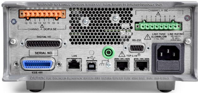
2601-PULSE rear panel.
