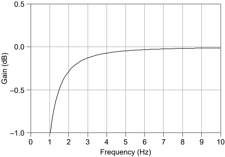
Figure 2. AC Cutoff Frequency Response
