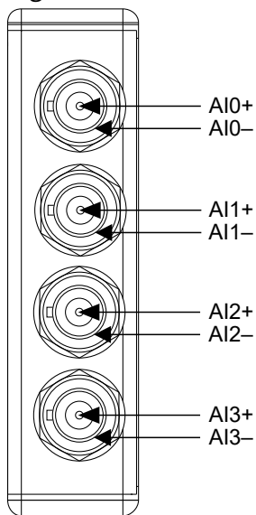
Figure 1. NI-9234 Pinout
