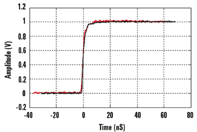
N2792A Differential Step Response
