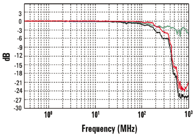
Figure 3. V_{out}/V_{in} vs. Frequency response of N2792A/N2818A (red = V_{out}/V_{in} , green = V_{in} , black = V_{out} )
