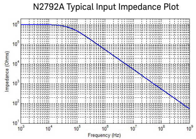
Figure 6. Input impedance vs. Frequency of N2792A/N2818A
