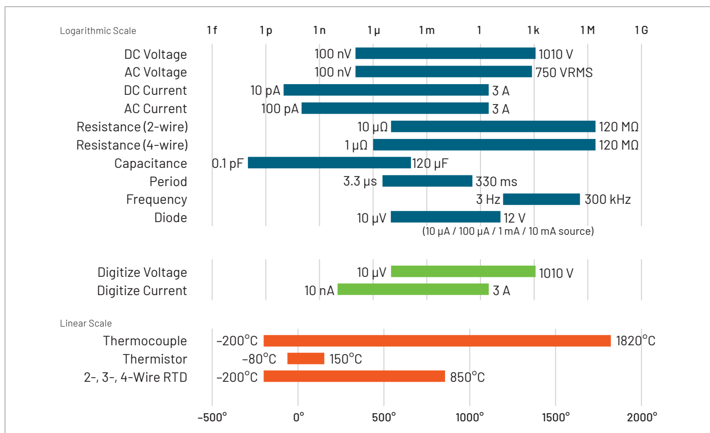
DAQ6510's 15 measurement functions and ranges.
