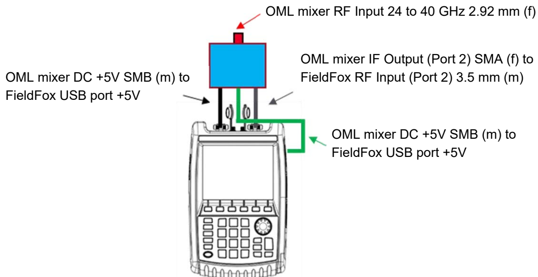
Figure 1. OML external mixer diagram 1
