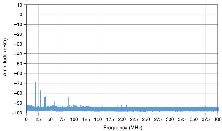
Figure 9. 10 MHz Single-Tone Spectrum [23] , Measured
