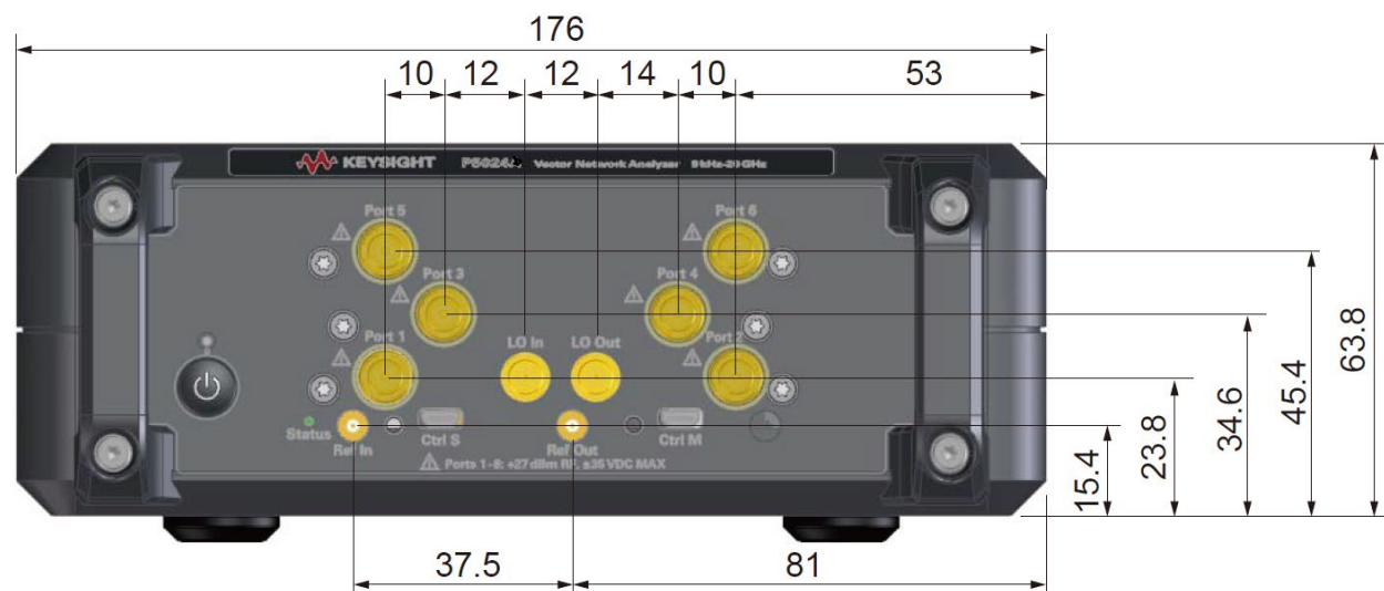
Dimensions (front view, P5020B/21B/22B/23B/24B with option 600, in millimeters)
