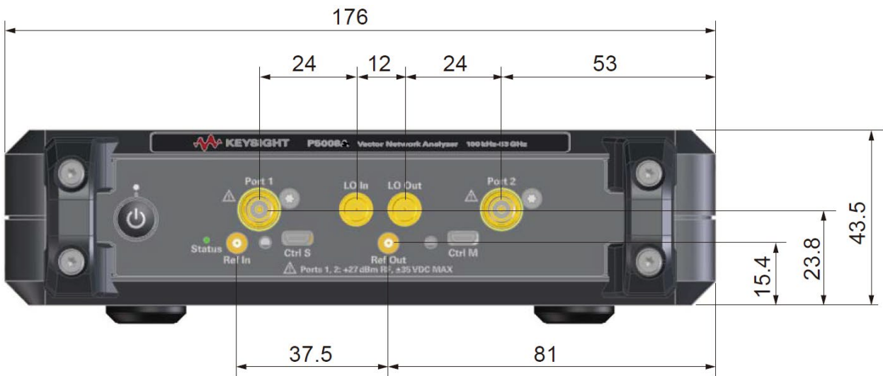
Dimensions (front view, P5000B/01B/02B/03B/04B/05B/06B/07B/08B with option 200, in millimeters)
