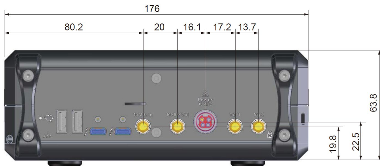
Dimensions (rear view, P5020B/21B/22B/23B/24B/25B/26B/27B/28B with option 400 or 402, or P5020B/21B/22B/23B/24B with option 600, in millimeters)
