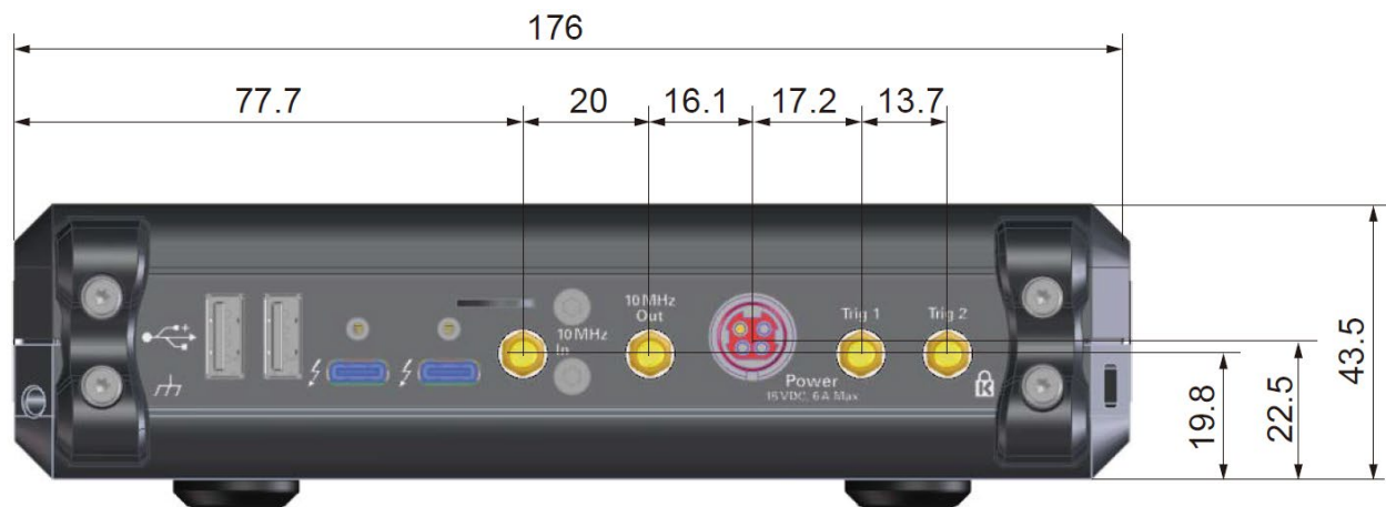
Dimensions (rear view, P5000B/01B/02B/03B/04B/05B/06B/07B/08B with option 200, in millimeters)
