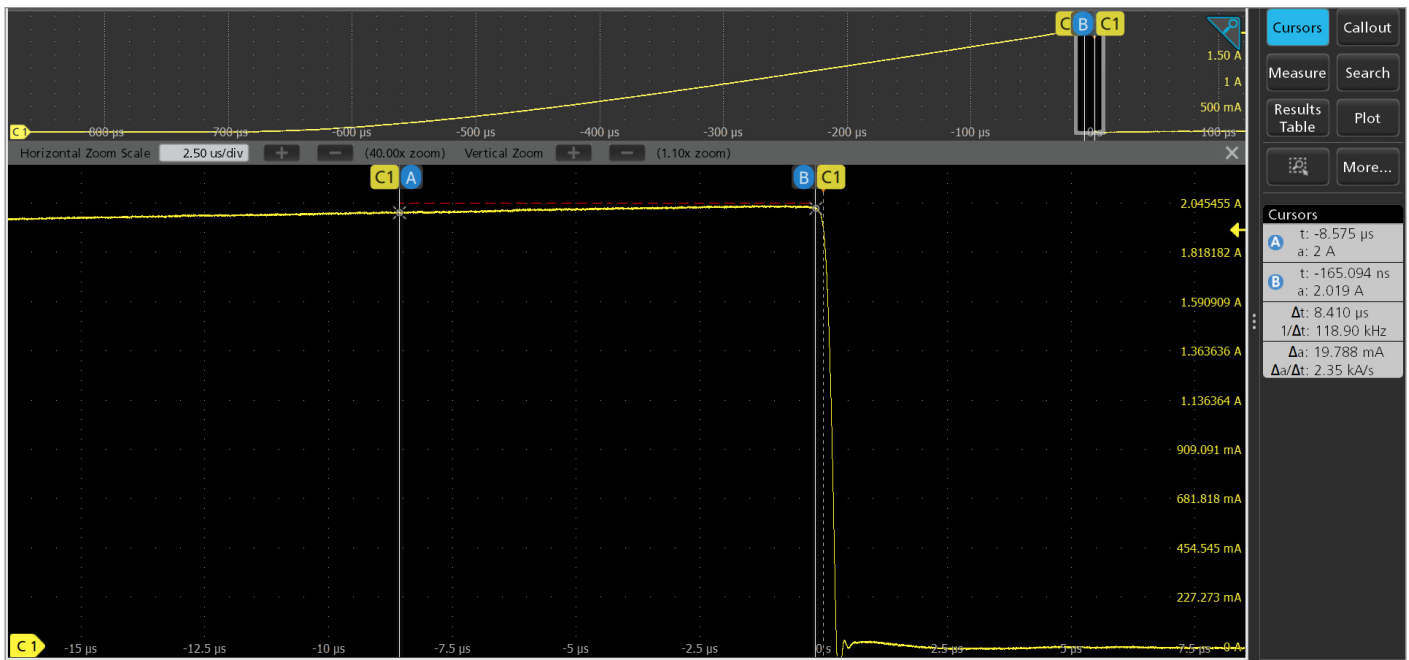
Figure 10: MPSU50-2ST OCP Response Time <50µsec
