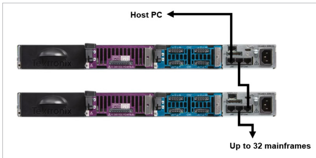
Figure 13: Scaling MP5000 with TSP-Link
