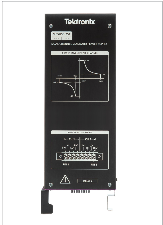
Figure 9: MPSU50-2ST Module: Dual Channel PSU
