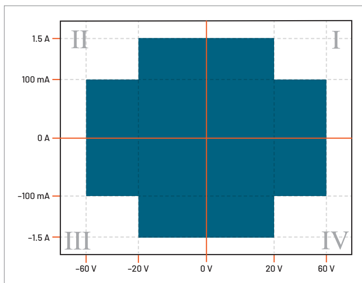
Figure 14: MSMU60-2 Power Envelope
