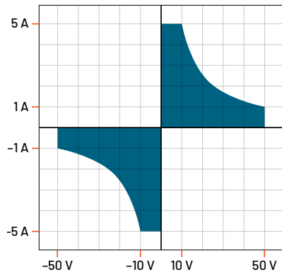
Figure 16: MPSU50-2ST Power Envelope
