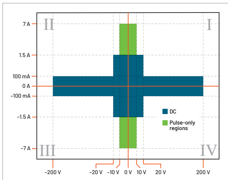
Figure 15: MSMU200-2 Power Envelope 3
