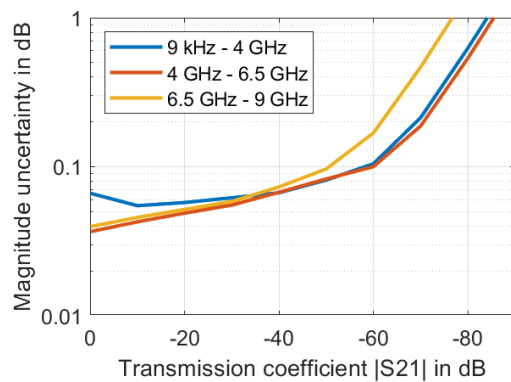
Typical uncertainty of transmission magnitude and transmission phase measurements for the R&S®ZNB3004 with or without frequency upgrade option, in the frequency range from 9 kHz to 9.0 GHz; analysis conditions: S_{11} = S_{22} = 0 , calibration power: –10 dBm, measurement power: –10 dBm
