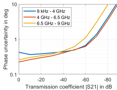
Typical uncertainty of transmission magnitude and transmission phase measurements for the R&S®ZNB3004 with or without frequency upgrade option, in the frequency range from 9 kHz to 9.0 GHz; analysis conditions: S_{11} = S_{22} = 0 , calibration power: –10 dBm, measurement power: –10 dBm
